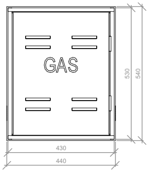
VISTA FRONTAL
